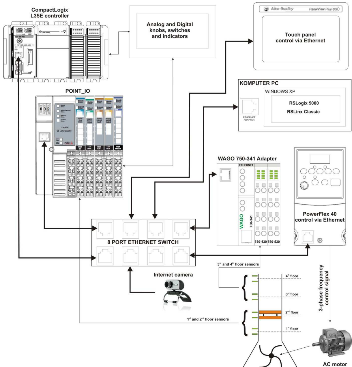
Fig. 1: Schematic diagram of the laboratory setup
