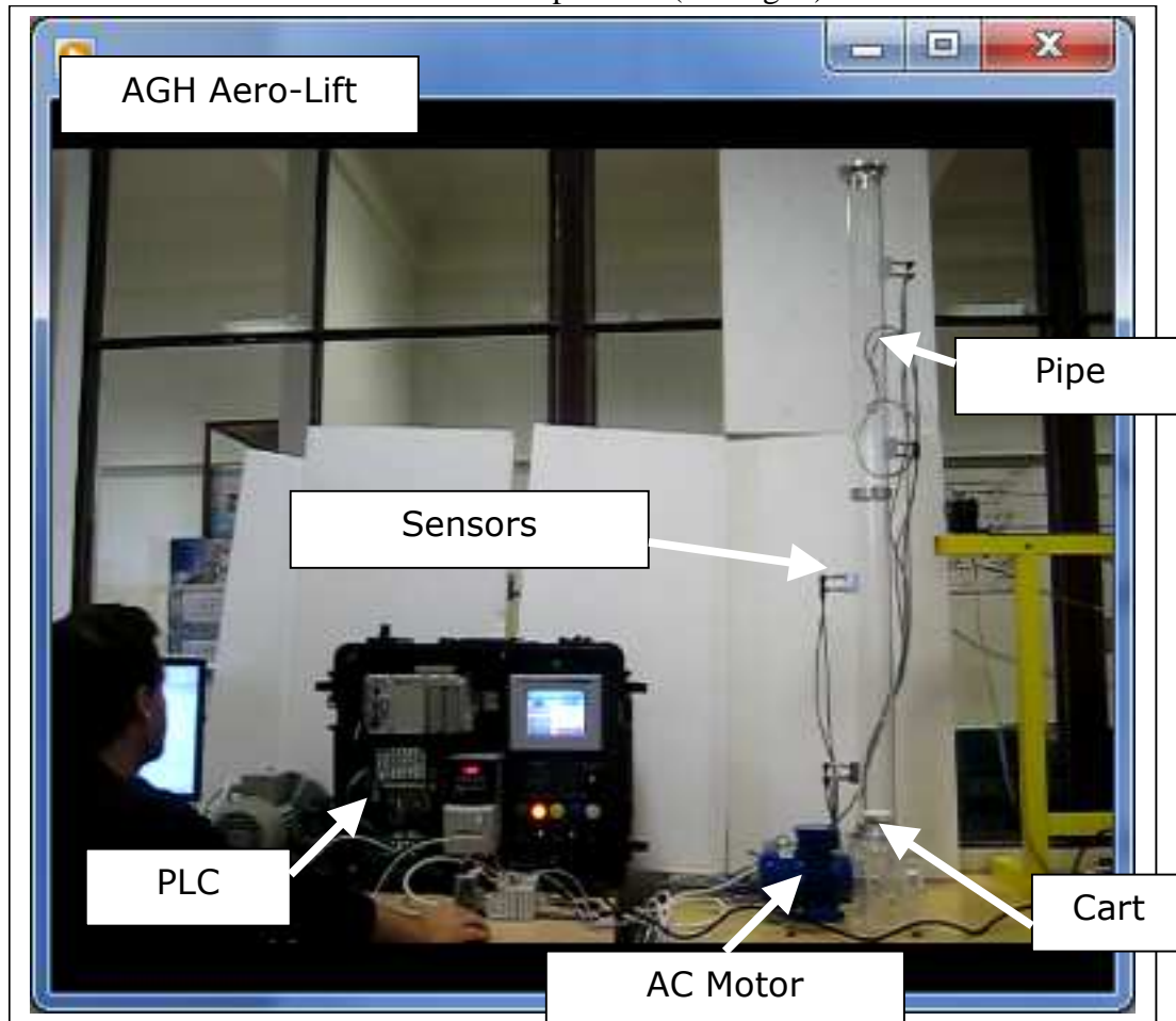
Fig. 2: Aero-Lift - laboratory test-rig
