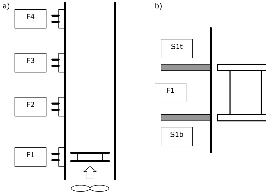
Fig. 3: Aero-Lift test rig: a) system overview, b) floor configuration
